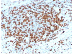
Immunohistochemical analysis of formalin-fixed, paraffin-embedded human tonsil using Anti-CD3 epsilon Antibody [C3e/3125R].
