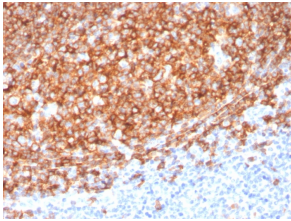
Immunohistochemical analysis of formalin-fixed, paraffin-embedded human tonsil using Anti-CD20 Antibody [MS4A1/3410].
