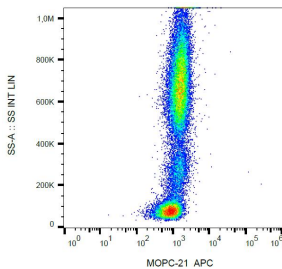
Example of non-specific Mouse IgG1 (A86198) signal on human peripheral blood; surface staining, 3 µg/ml.
