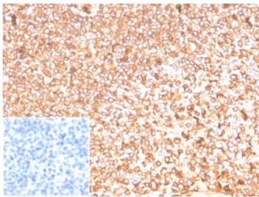
Immunohistochemical analysis of formalin-fixed, paraffin-embedded human tonsil tissue using Anti-beta Actin Antibody [ACTB/1109]. Inset: PBS instead of the primary antibody. Secondary antibody negative control.
