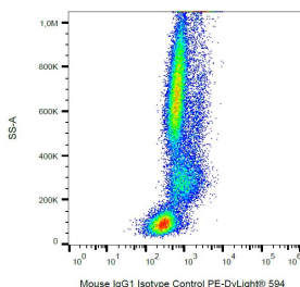
Example of non-specific Mouse IgG1 (A86201) signal on human peripheral blood; surface staining, 1 µg/ml.
