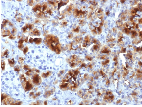
Immunohistochemical analysis of formalin-fixed, paraffin-embedded human pancreas using Anti-Glycoprotein 2 Antibody [GP2/1712].
