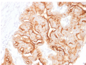
Immunohistochemical analysis of formalin-fixed, paraffin-embedded human ovarian carcinoma using Anti-MUC16 Antibody [MUC16/1860].
