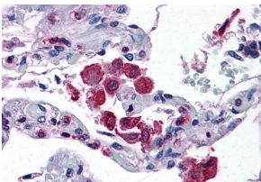
Anti-ALOX5AP Antibody (A84031) (3.75µg/ml) staining of paraffin embedded Human Lung. Steamed antigen retrieval with citrate buffer pH 6, AP-staining.
