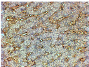
Anti-APOA1 Antibody (A84551) (2µg/ml) staining of paraffin embedded Human Liver. Steamed antigen retrieval with citrate buffer pH 6, HRP-staining.
